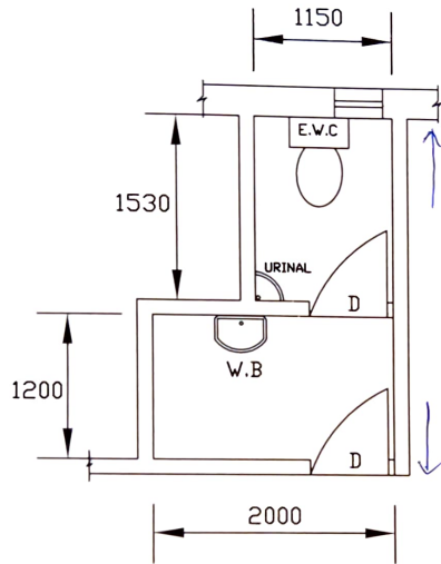
EXISTING COMPUTER SECTION TOILET
