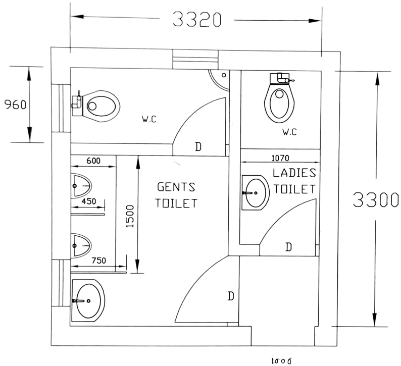
PROPOSED PLAN OF TOILET BLOCK
